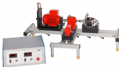
AT 200 - Determination of gear efficiency
