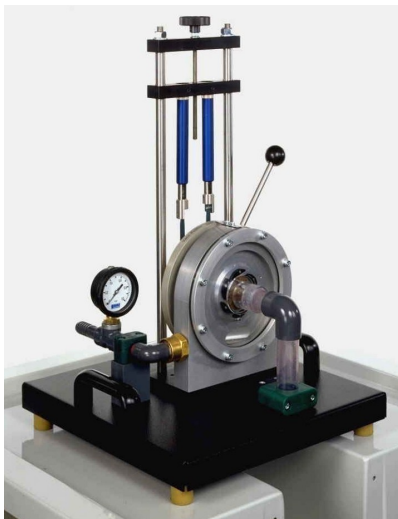
HM150.20 Operating Principle of a Francis Turbine
