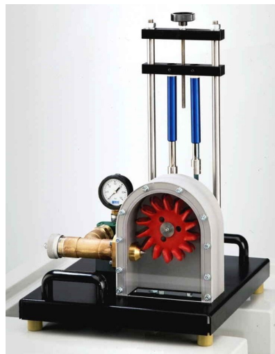
HM150.19 Operating Principle of a Pelton Turbine
